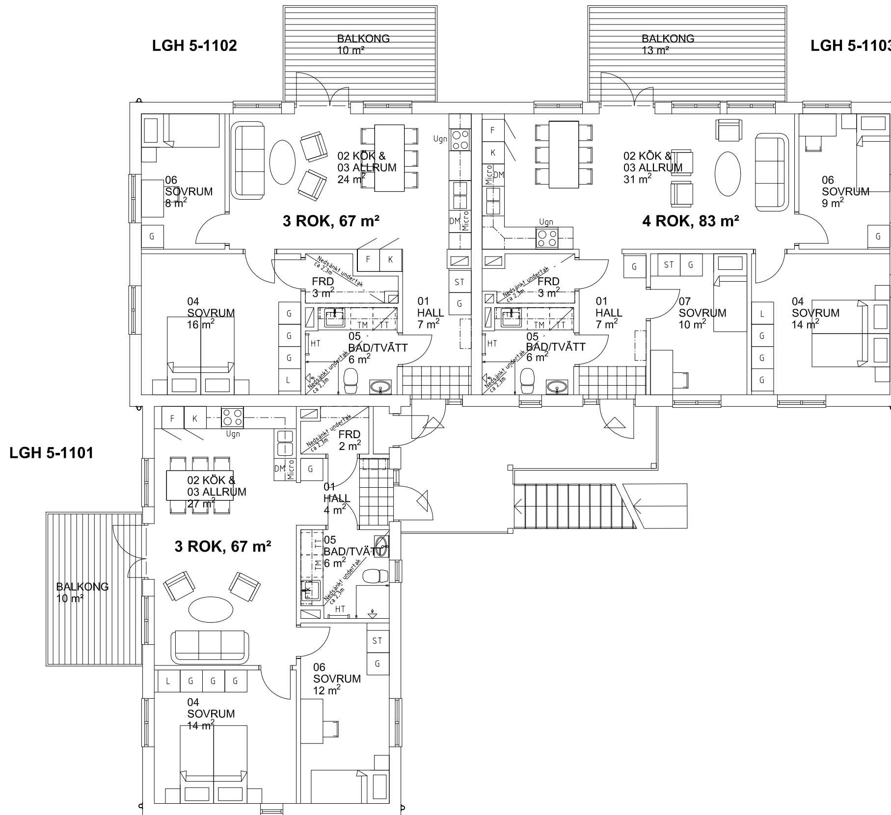
PLAN 2 LGH 5-1101/1102/1103
