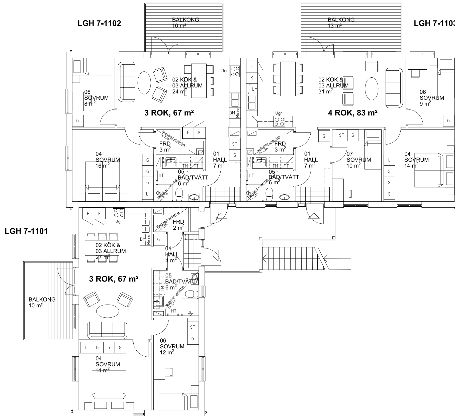
PLAN 2 LGH 7-1101/1102/1103
